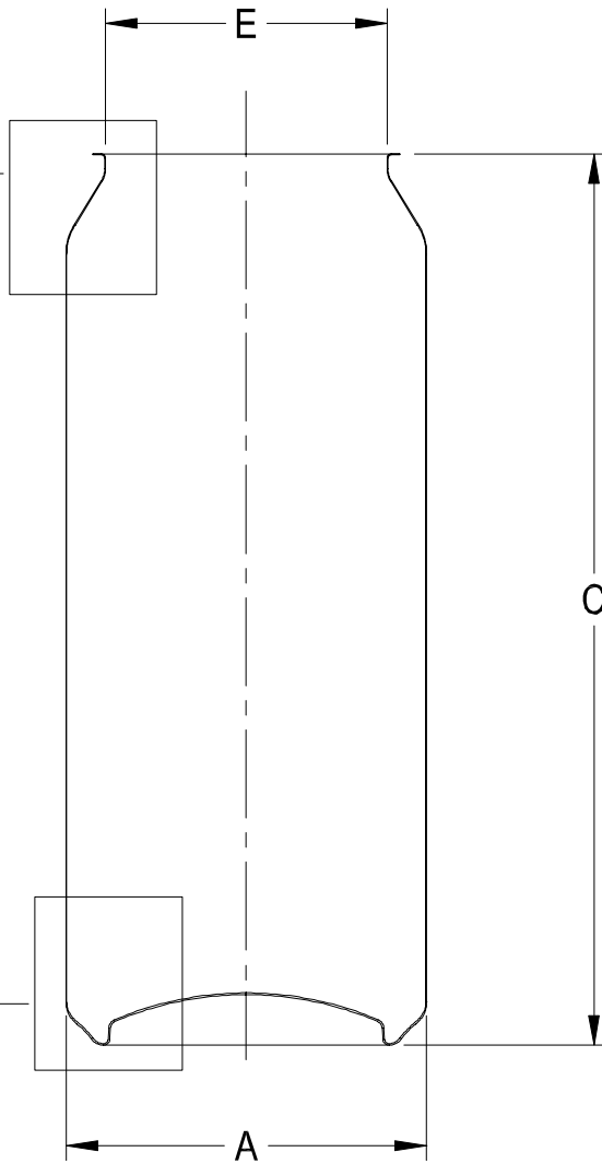
NECKED & FLANGED CAN
